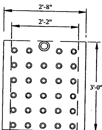
32PS (Section) is 32"OD/26"ID 36" Overall Height
