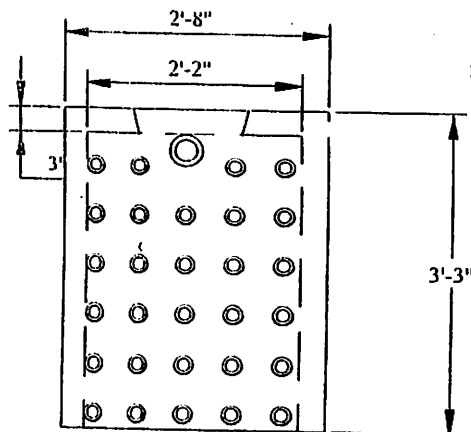
32P (Cover Cast) is 32"OD/26"ID 39" Overall Height
